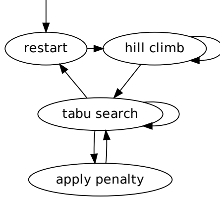
Figure 7: The generalised local search machine (GLSM) [2] of our tabu search heuristic.
