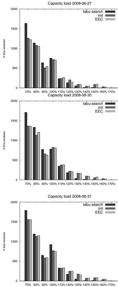
Figure 11: The capacity balance \frac{demand[a,t]}{cap_a} , with values outside the closed interval [70\%, 170\%] omitted, on the training flight plans for three different contingency plans, an empty contingency plan (init), a contingency plan generated by our tabu heuristic (tabu), and a contingency plan generated by EUROCONTROL (EEC). A favourable distribution would be heavy around 100% and decrease with distance, faster on the right-side (overcapacities) than on the left-side (undercapacities). The reason this is not the case for undercapacities is because during non-rush hours there are not enough flights to fully utilise the airspace, hence undercapacities are inevitable.
