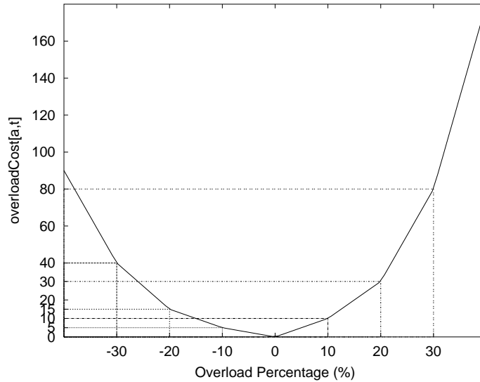
Figure 6: Piecewise linear function giving the overcapacity cost overcapacityCost[a, t] in terms of the overcapacity percentage.
