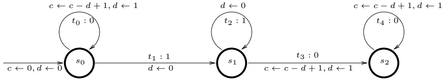
Figure 1. Automaton associated with the global_contiguity constraint, with initial state s_0 , final states s_0, s_1, s_2 , and transitions t_0, t_1, t_2, t_3, t_4 labelled by values 0 or 1. The missing transition for value 1 from state s_2 is assumed to go to a dead state. The automaton has been annotated with counters [2]: the final value of counter c is the number of stretches of value 0, whereas d is an auxiliary counter.
